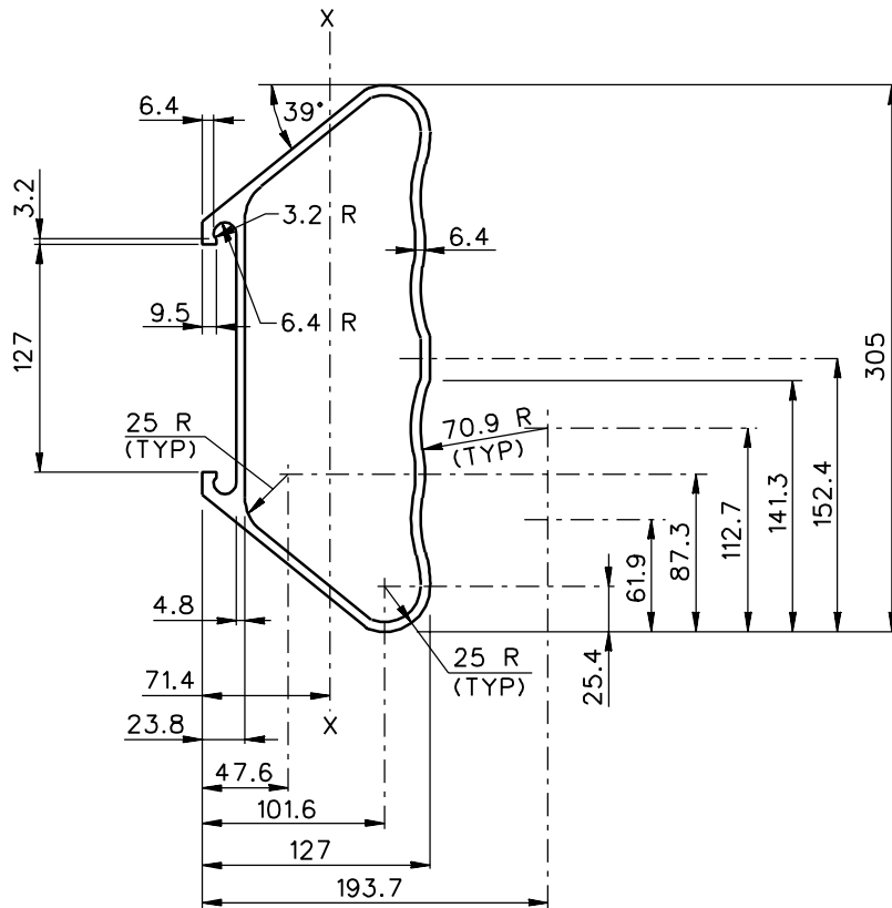
SECTION
