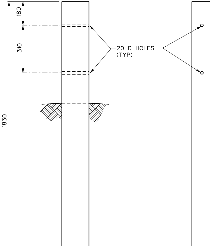
SIDE
