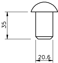
NOMINAL 21 HIGH BUTTON-HEAD RIVET
